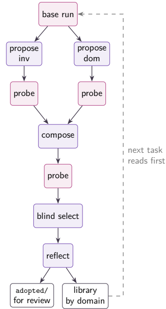
Figure 1: One round of refine . Pink stages run the task through ac run ; purple stages are Claude sessions reading evidence served as files. A candidate identical to an earlier harness reuses its run.
