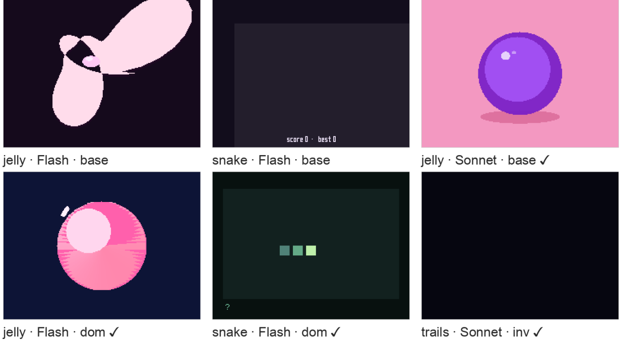
Figure 2: The last frame ac check recorded for six runs; a tick marks the chosen piece. Left: the R1 jelly base folds into lobes under a poke where the adopted candidate dents and holds. Middle: the R1 snake base reaches game over before any input; the adopted candidate waits. Right: Sonnet 5.5’s jelly base, chosen over both candidates, and its chosen trails piece, blank because the frame was taken after the trail faded — the case its adopted rule names.
