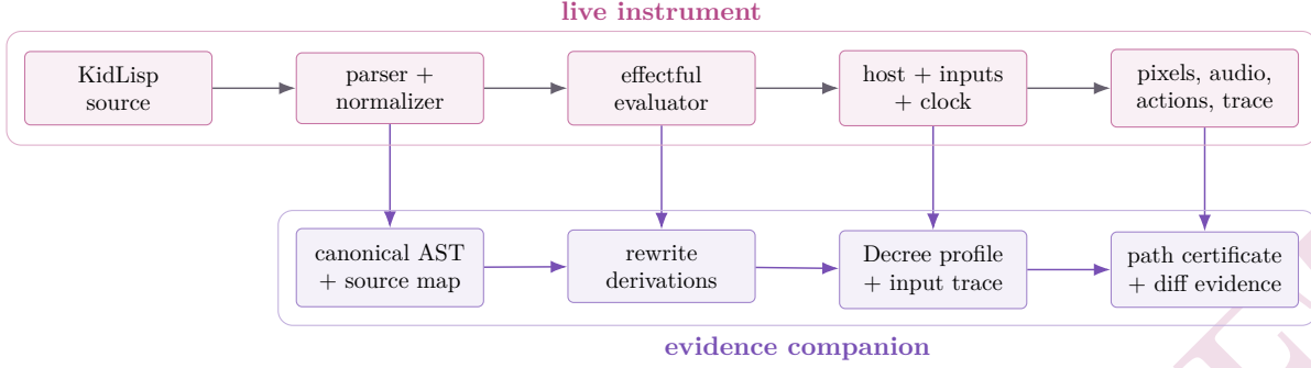
Figure 2: The proposed architecture. The live instrument remains permissive and immediate. A companion lane records normalization, rewrite derivations, host and input indices, observations, and bounded equivalence certificates. The two lanes meet at explicit taps; the checker never has to sit inside the paint loop.
