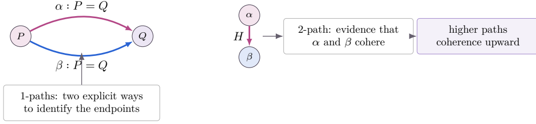
Figure 1: The identity ladder used in this study. P and Q are endpoints; \alpha and \beta are distinct witnesses that identify them; H identifies those witnesses. For KidLisp the picture is initially a design vocabulary, not a constructed HoTT model: source rewrites and render tests do not automatically satisfy the laws required of path types.
