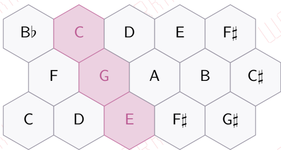
Figure 3: Wicki–Hayden hex layout (Wicki 1896 / Hayden 1986). Same-row neighbors differ by a whole tone; up-and-right neighbors by a perfect fourth. The C major triad ( C E G ) is highlighted: the chord is a fixed three-cell shape on the surface, and translating that shape transposes the chord to any key. “Transposition is translation” is the central isomorphic-keyboard claim, and the property the standard piano’s white-and-black asymmetry sacrifices.
