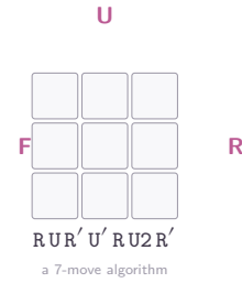
Figure 7: Singmaster’s cube notation [Singmaster, 1981]. Each capital letter names a face (Up, Down, Left, Right, Front, Back); a bare letter is a clockwise quarter-turn, a primed letter (') a counter-clockwise quarter-turn, and a digit-2 a half-turn. The seven-token string R U R' U' R U2 R' is a complete algorithm portable between cubers, GitHub repos, and YouTube tutorials — the keymap-notation pair traveling as text.
