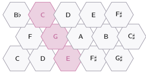
Figure 3: Wicki–Hayden hex layout (Wicki 1896 / Hayden 1986). Same-row neighbors differ by a whole tone; up-and-right neighbors by a perfect fourth. The C major triad ( C E G ) is highlighted: the chord is a fixed three-cell shape on the surface, and translating that shape transposes the chord to any key. “Transposition is translation” is the central isomorphic-keyboard claim, and the property the standard piano’s white-and-black asymmetry sacrifices.
