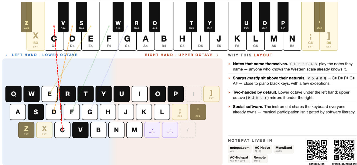
Figure 1: The notepat.com keymap. The QWERTY letter c plays C, d plays D, ..., b plays B; the upper octave continues alphabetically ( h i j k l m n ); sharps sit above their natural by piano-black-key analogy where possible. Two-handed split: lower octave on left hand, upper on right. Implementations: notepat.com (web), AC Native, MenuBand (macOS menubar), AC-Notepat (Max for Live), Remote (phone).
