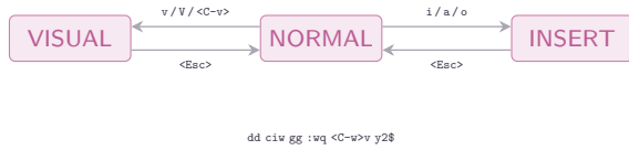
Figure 6: Vim’s modal keymap and its travelling notation. Modes (NORMAL, INSERT, VISUAL) are connected by labeled keystroke transitions; common commands ( dd delete-line, ciw change-inner-word, gg go-top, :wq write-and-quit, etc.) are the discursive currency of the keymap. The notation is so portable it has been re-implemented in VS Code, JupyterLab, Vimium, the macOS Cocoa text system, and set -o vi .
