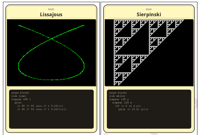
Figure 4: “Lissajous” (math curves) and “Sierpinski” (bitwise AND fractal).
