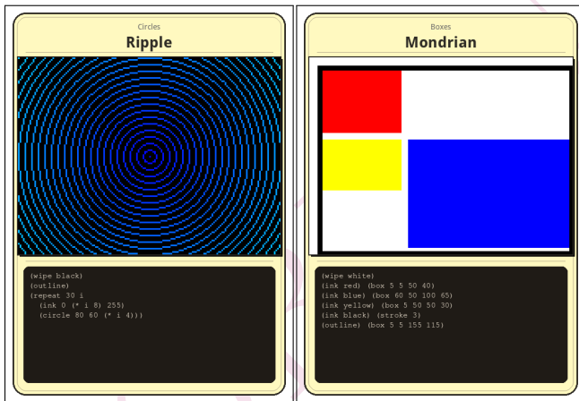
Figure 3: “Ripple” (circles) and “Mondrian” (boxes).
