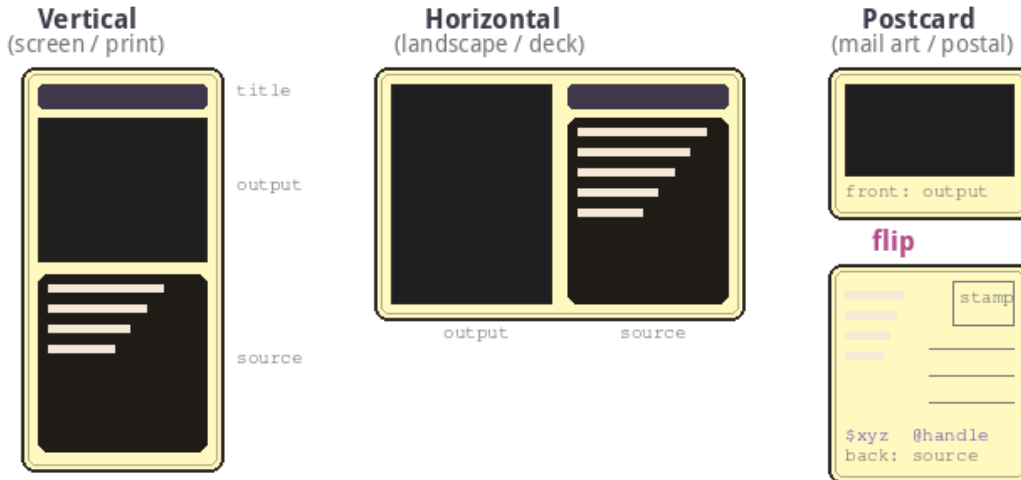
Figure 8: Three layout strategies. Vertical: title / image / source stacked top-to-bottom, optimized for phone screens and portrait printing. Horizontal: image on the left, title and source on the right, suited for landscape cards and side-by-side deck browsing. Postcard: rendered output on the front, source code and metadata on the back—a mailable card where the program is hidden until you flip it over.
