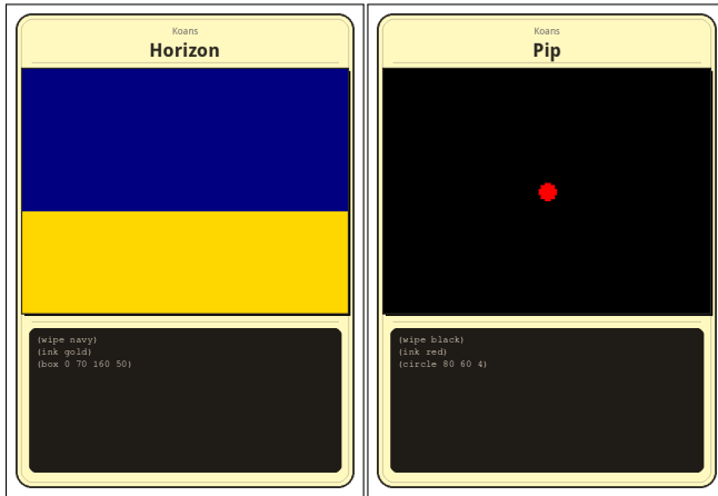
Figure 6: “Horizon” and “Pip” — minimal koans (2–3 lines each).
