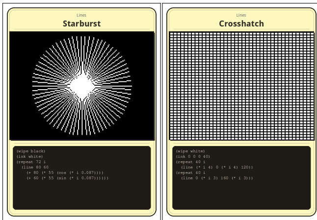
Figure 2: “Starburst” and “Crosshatch” — line cards.
