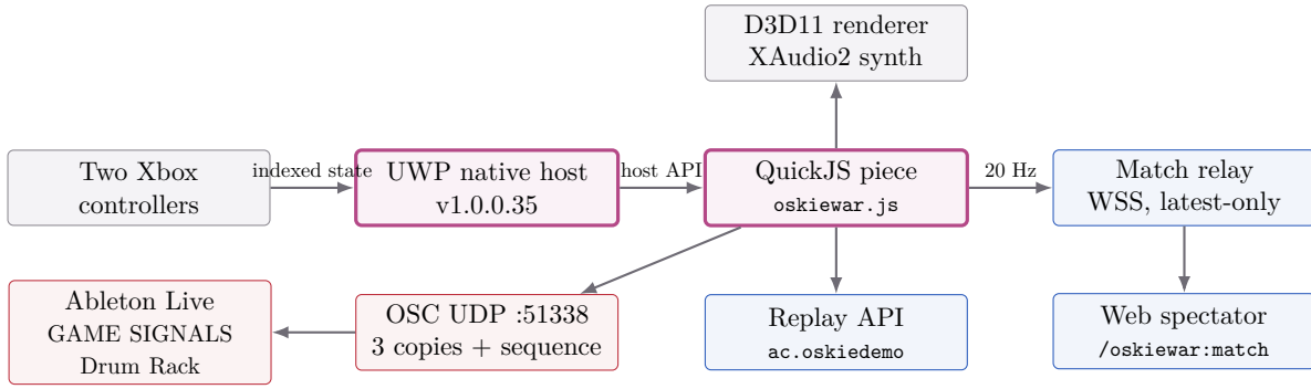
Figure 1: The native shell owns privileged I/O; browser spectators receive bounded state through the relay and never connect to the console directly.
