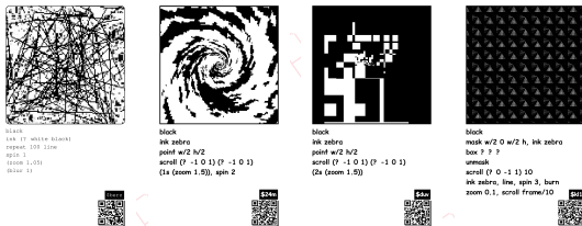
Figure 3: Repertoire as printable cards. Four KidLisp pieces— $berz , $24m , $duv , $kl1 —each a self-contained program that runs on AC Native OS as the laptop’s whole operating system. The pixel image at top is the live output; the source code beneath is the entire program (no imports, no build step). The QR code links to the live piece on Aesthetic.Computer, where 17,000+ KidLisp programs already exist as a shareable repertoire. PLork’s repertoire was a closed library of compositions performed by enrolled students; AC Native OS’s repertoire is a public folk process: forkable, URL-addressable, six lines long.
